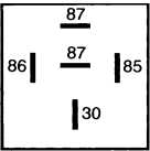
Normally-open relay with dual output
